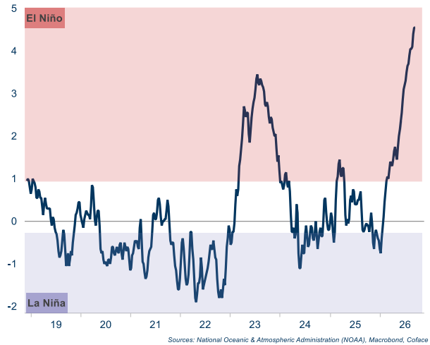
Figure 3. El Niño index (ocean surface temperature, anomalies 1+2, in °C)
